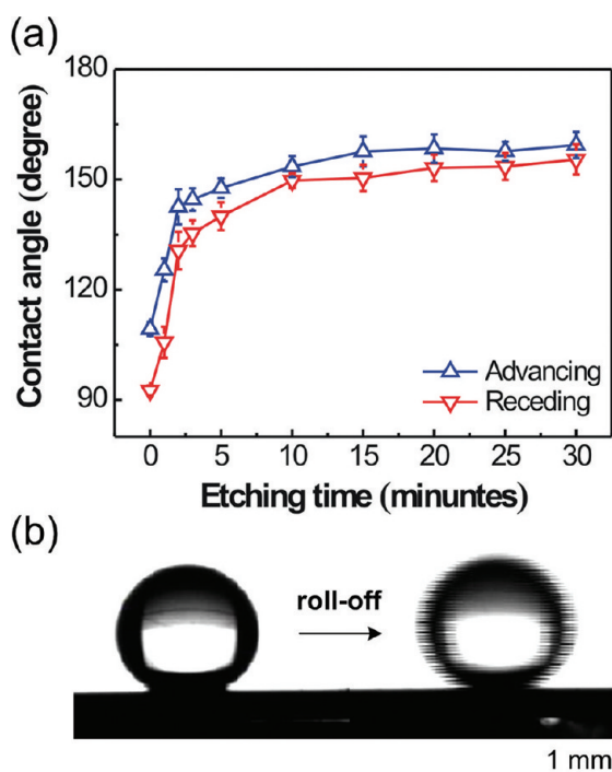
Figure 2. (a) Advancing and receding water CAs of surface modified Si NW arrays as a function of t_e . (b) Water droplet on a surface-modified Si NW array (left). The water droplet easily rolled off in the absence of any tilt angle, and the droplet edge is blurred because of the fast movement of the water droplet (right).
