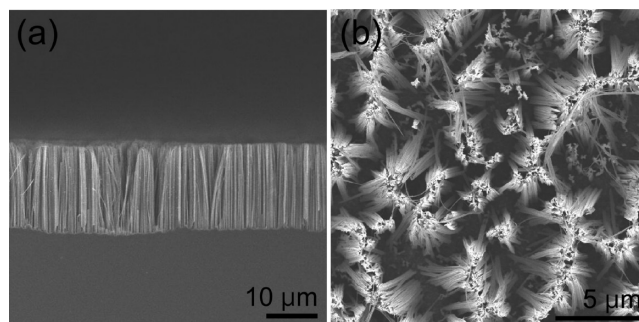
Figure 1. Typical SEM images of (a) cross-sectional and (b) top views of Si NWs fabricated using the AEE method with a t_e of 30 min.
