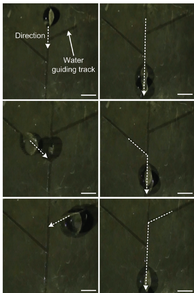
Figure 8. Sequential photographs of water droplets on cross-linked hydrophilic water guiding tracks. The scale bars in the images indicate 3 mm.
