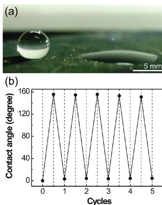
Figure 5. (a) Photograph of the wettability contrast between the DTS-coated region (left) and UV-treated region on the same substrate with Si NW arrays. (b) Reversible wettability conversion of the Si NW arrays between superhydrophobic and hydrophilic was achieved by repeating the coating and decomposition process of DTS.
