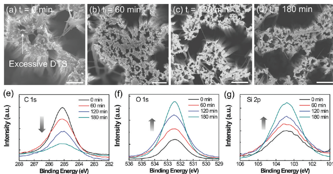
Figure 4. Typical top-view SEM images of the DTS-coated Si NW arrays at (a) t_i = 0 min, (b) t_i = 60 min, (c) t_i = 120 min, and (d) t_i = 180 min. The scale bars in the images indicate 1 \mu\text{m} . XPS spectra of (e) C 1s, (f) O 1s, and (g) Si 2p for the DTS-coated Si NW arrays of which t_i was varied from 0 to 180 min.
